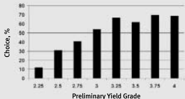
Fig. 2: Choice distribution
